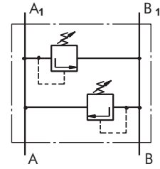
Dual Crossover Relief Valve type KPDW ...
